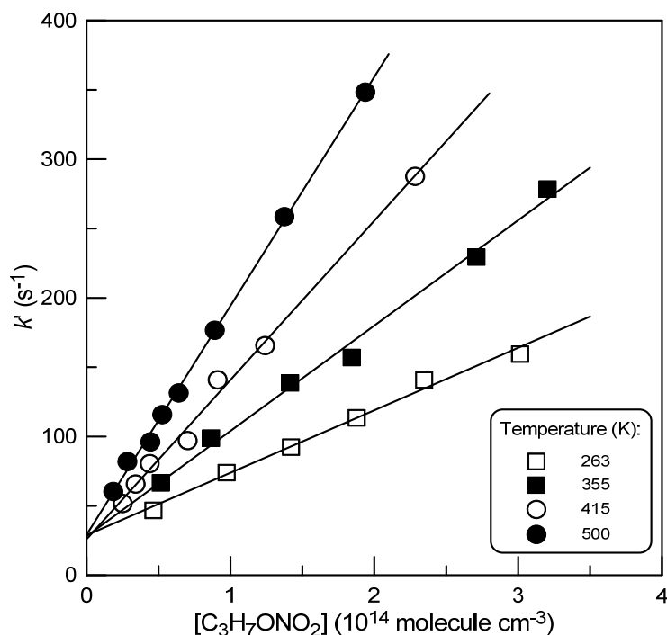
Figure 3 Example of pseudo-first order plots obtained from OH decay kinetics in excess of propyl nitrate.
