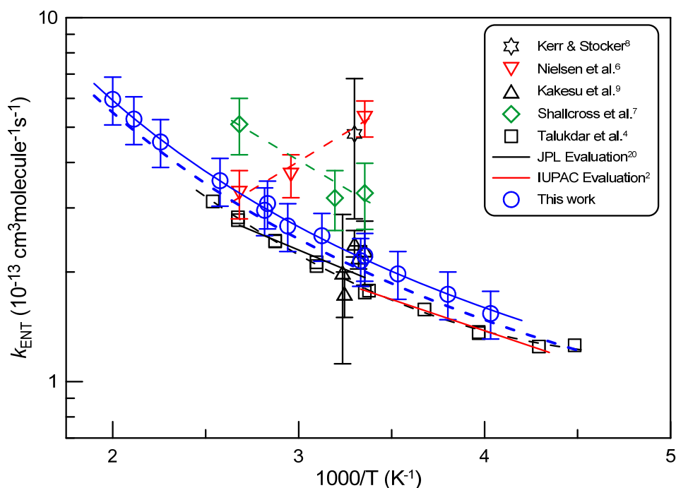
Figure 4 Summary of the measurements of the rate constant of the reaction OH + ethyl nitrate.
