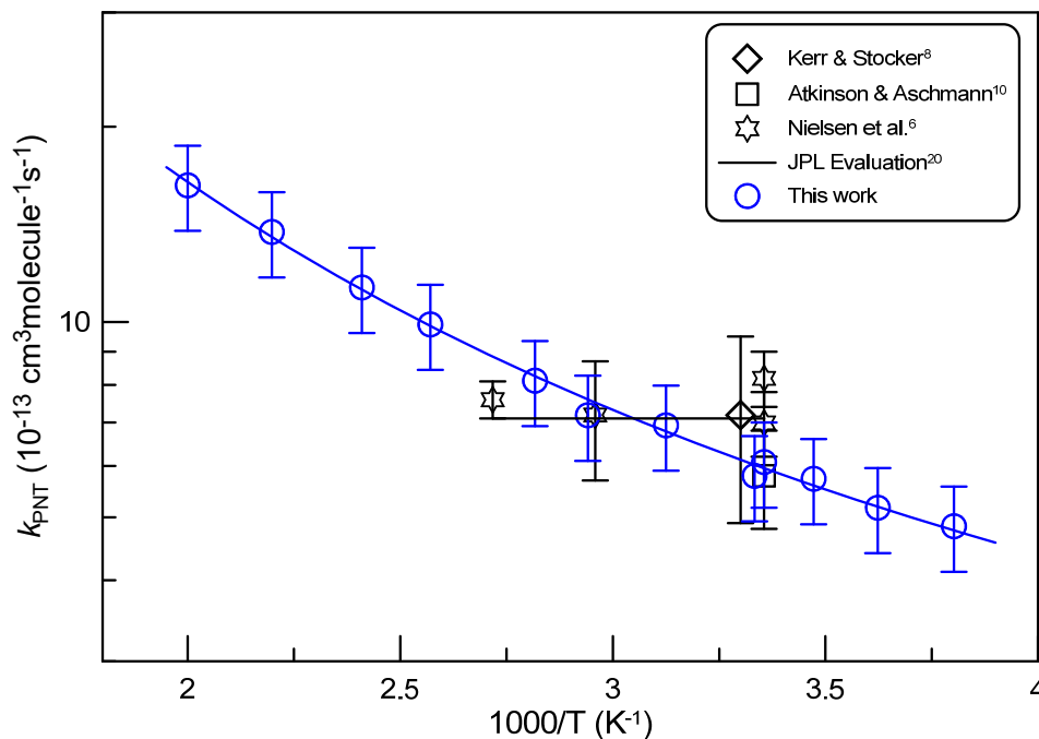
Figure 5 Summary of the measurements of the rate constant of the reaction OH + propyl nitrate.
