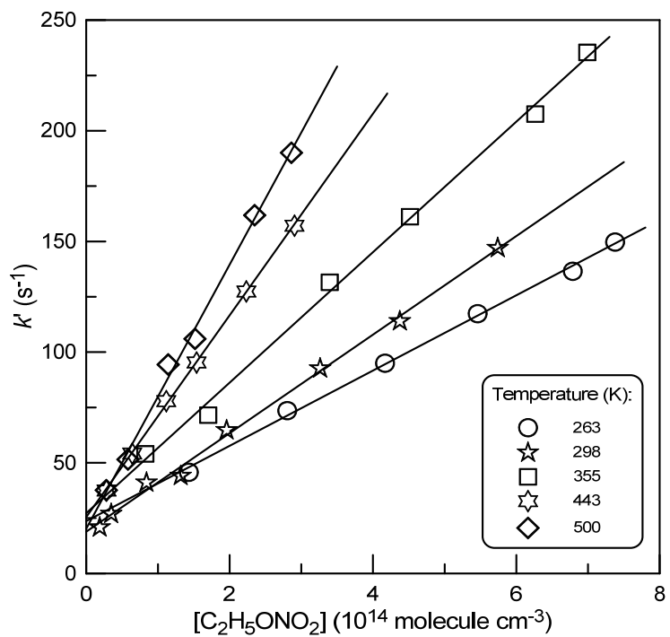
Figure 2 Example of pseudo-first order plots obtained from OH decay kinetics in excess of ethyl nitrate.
